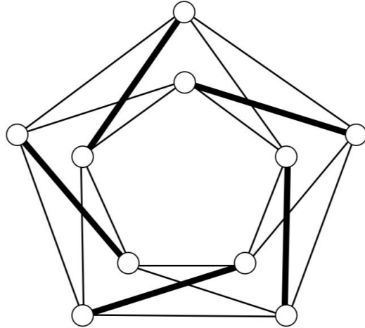
Figure 1: C_5^2 with a clique cover shown as thick edges.
